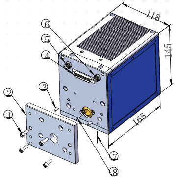
PSH14AW Scan Head
